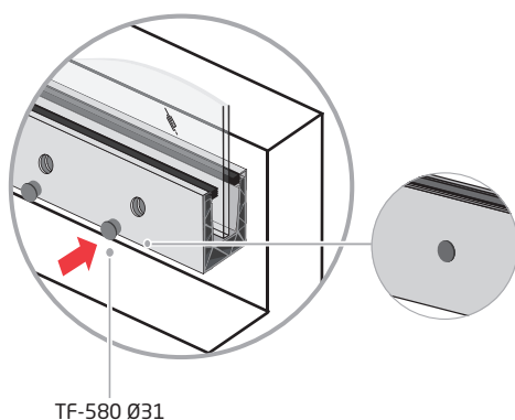
SV-1602 Side Inverse TF-580
